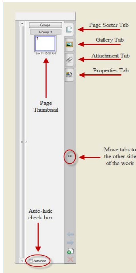
Figure 1. Side tab toolbar in SMART Notebook software
