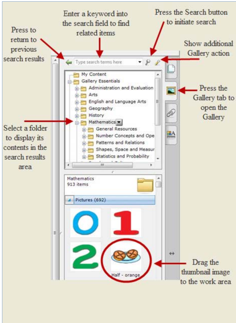
Figure 2. Notebook software Gallery
