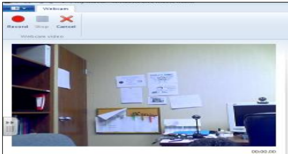
Figure 2. Webcam view
