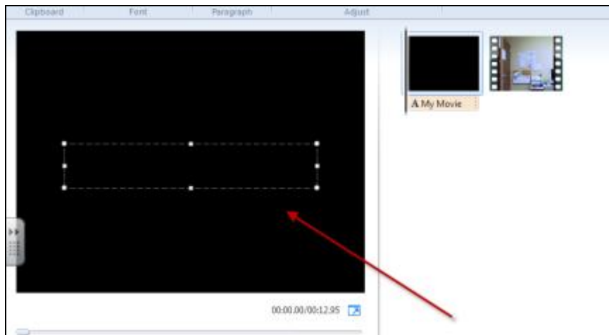
Figure 14. Add Title
