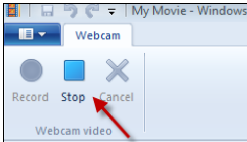
Figure 4. Stop button
