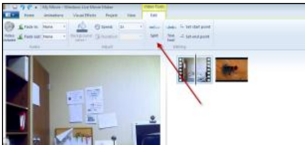
Figure 9: Split command
