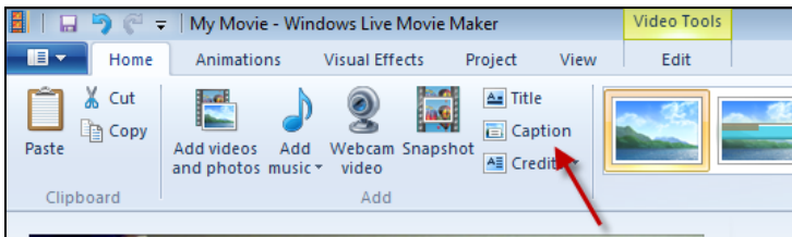
Figure 11. Caption command
