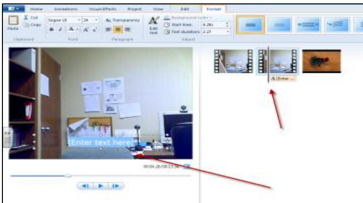
Figure 12. Adding captions
